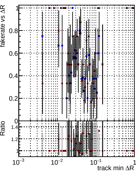
Fake rate vs \Delta R (track, jet) DQM_V0001_R000000001 Global cmssw1000time RECO DQM_V0001_R000000001 Global mkFitNewOLD1000time RECO DQM_V0001_R000000001 Global mkFitNewBins2DC1000time RECO
