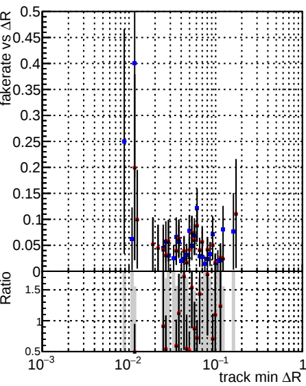
DQM_V0001_R000000001 Global cmssw1000time_RECO DQM_V0001_R000000001 Global mkFitNewOLD1000time_RECO DQM_V0001_R000000001 Global mkFitNewBins2DC1000time_RECO
