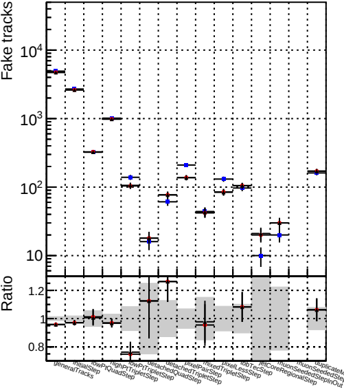
Legend Series Name Model Fit Type Number DQM_V0001_R0000000001_Global_cmssw1000time_RECO Global cmssw1000time_RECO DQM_V0001_R0000000001_Global_mkFitNewOLD1000time_RECO Global mkFitNewOLD1000time_RECO DQM_V0001_R0000000001_Global_mkFitNewBins2DC1000time_RECO Global mkFitNewBins2DC1000time_RECO
