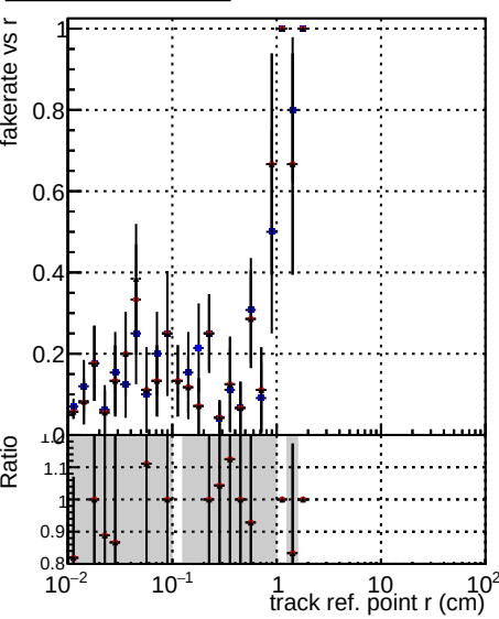
DQM_V0001_R000000001 Global cmssw1000time RECO DQM_V0001_R000000001 Global mkFitNewOLD1000time RECO DQM_V0001_R000000001 Global mkFitNewBins2DC1000time RECO
