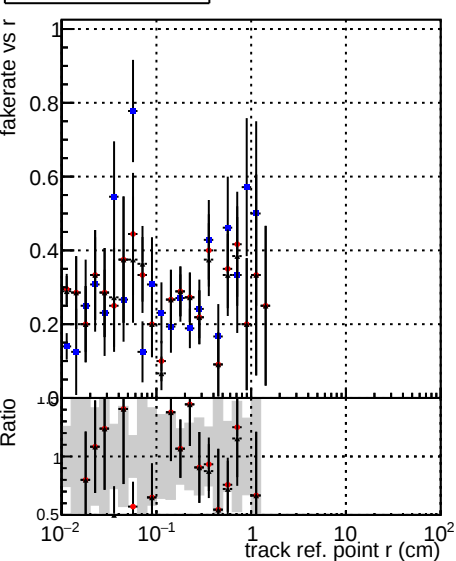
Fake rate vs vertpos Legend: DQM_V0001_R000000001 Global cmssw1000time_RECO DQM_V0001_R000000001 Global mkFitNewOLD1000time_RECO DQM_V0001_R000000001 Global mkFitNewBins2DC1000time_RECO
