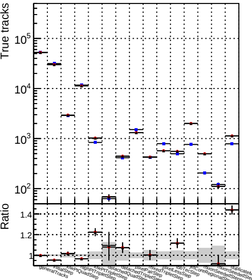
Number Legend Model Dataset Model DQM_V0001_R0000000001_Global_cmssw1000time_RECO DQM_V0001_R0000000001_Global_mkFitNewOLD1000time_RECO DQM_V0001_R0000000001_Global_mkFitNewBins2DC1000time_RECO
