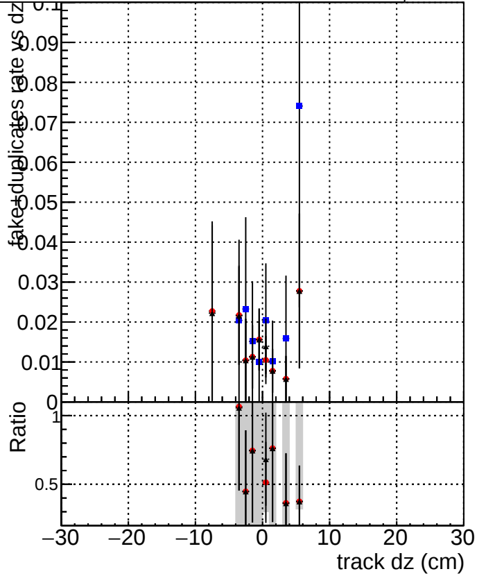
DQM_V0001_R000000001_Global_cmssw1000time_RECO DQM_V0001_R000000001_Global_mkFitNewOLD1000time_RECO DQM_V0001_R000000001_Global_mkFitNewBins2DC1000time_RECO
