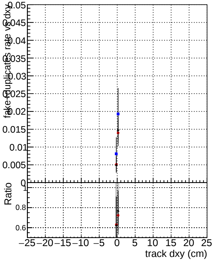
DQM_V0001_R000000001_Global_cmssw1000time_RECO DQM_V0001_R000000001_Global_mkFitNewOLD1000time_RECO DQM_V0001_R000000001_Global_mkFitNewBins2DC1000time_RECO
