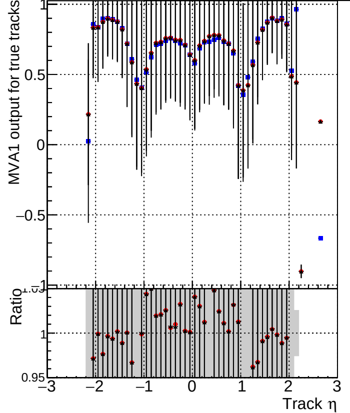
MVA1 of associated tracks (recoToSim) vs. track \eta Legend: DQM_V0001_R000000001_Global_cmssw1000time_RECO (blue squares) DQM_V0001_R000000001_Global_mkFitNewOLD1000time_RECO (red circles) DQM_V0001_R000000001_Global_mkFitNewBins2DC1000time_RECO (black triangles)
