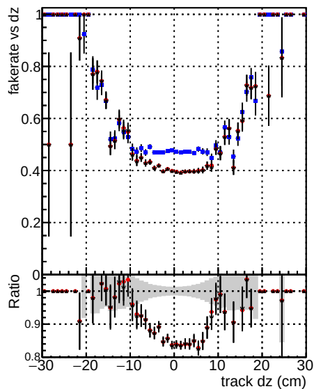
DOM V0001 R0000000001 Global cmssw1000time RECO DOM V0001 R0000000001 Global mktFitNewOld1000time RECO DOM V0001 R0000000001 Global mktFitNewBms2DC1000time RECO
