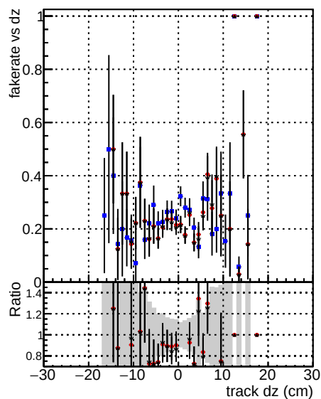
Fake rate vs dz DOM V0001 R0000000001 Global cms-sw1000time RECO DOM V0001 R0000000001 Global mkFitNewOLD1000time RECO DOM V0001 R0000000001 Global mkFitNewBms2DC1000time RECO
