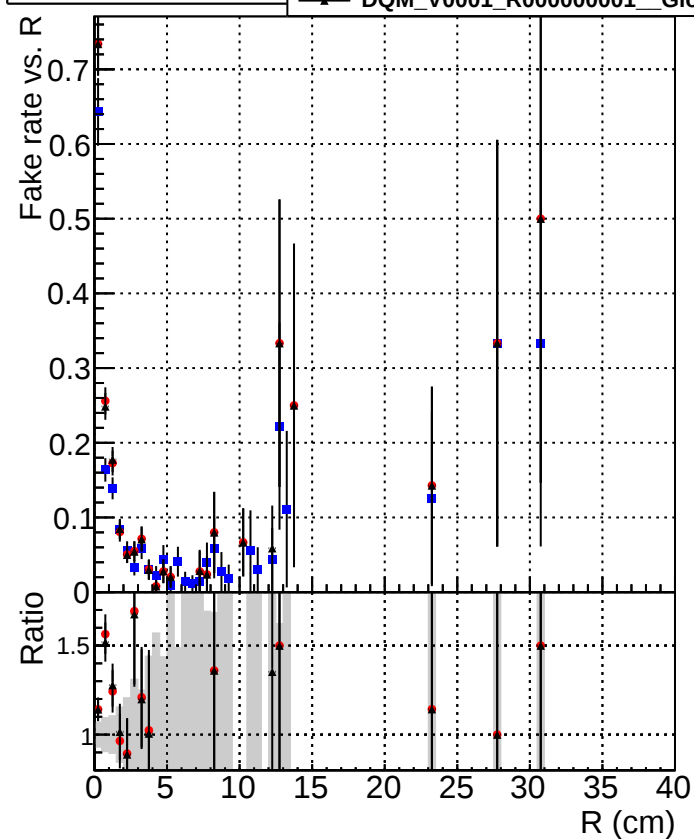
K_S^0 tracking fake rate
