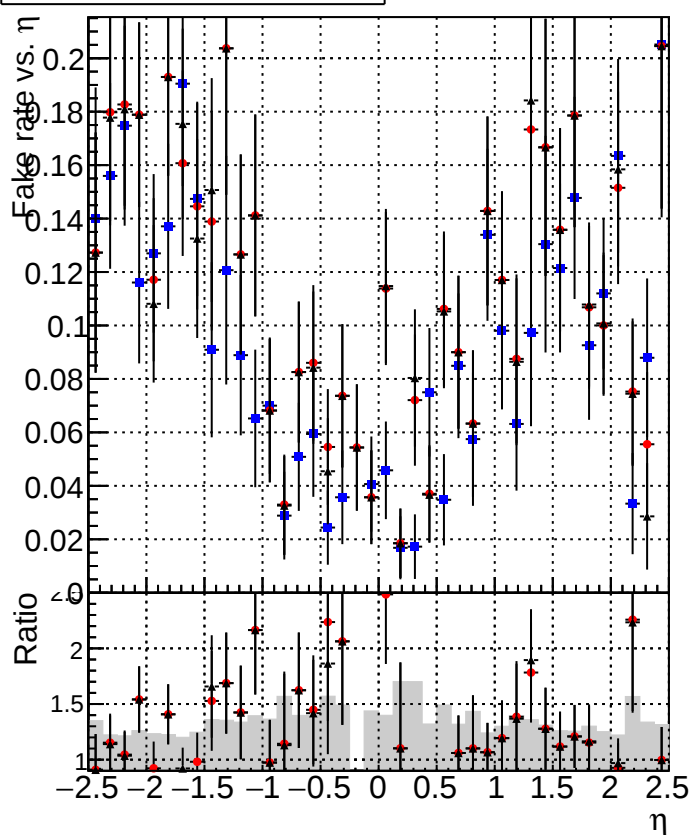
K_S^0 tracking fake rate vs \eta
