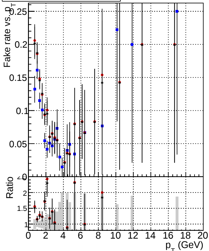
K_S^0 tracking fake rate vs p_T
