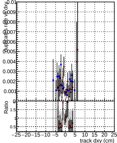
a|_mkFitNewOLD1000time RECO a|_mkFitNewBins2DC1000time RECO
