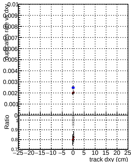
Global cmssw1000time RECO Global mktNewOldD1000 RECO Global mktNewBms2DC1000time RECO
