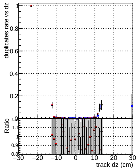
Global cmssw1000time RECO Global mkFitNewOldD1000time RECO Global mkFitNewBins2DC1000time RECO
