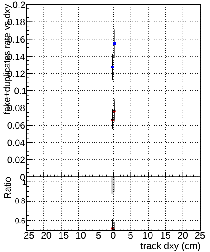
DQM_V0001_R0000000001_Global_cmssw1000time_RECO DQM_V0001_R0000000001_Global_mkFitNewOLD1000time_RECO DQM_V0001_R0000000001_Global_mkFitNewBins1DC1000time_RECO
