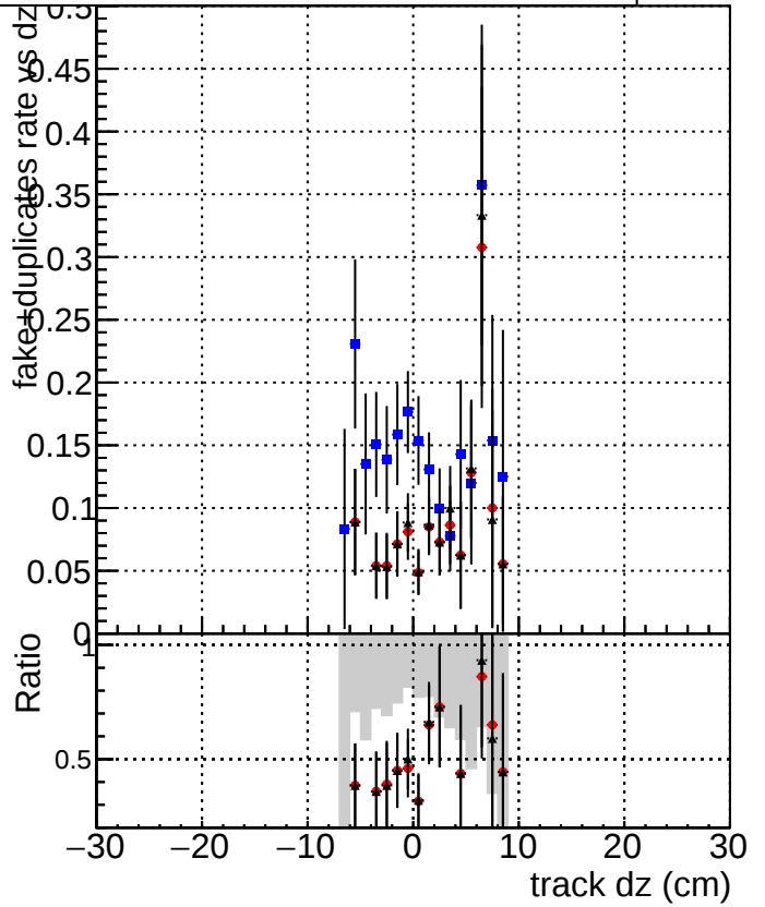
DQM_V0001_R0000000001_Global_cmssw1000time_RECO DQM_V0001_R0000000001_Global_mkFitNewOLD1000time_RECO DQM_V0001_R0000000001_Global_mkFitNewBins1DC1000time_RECO
