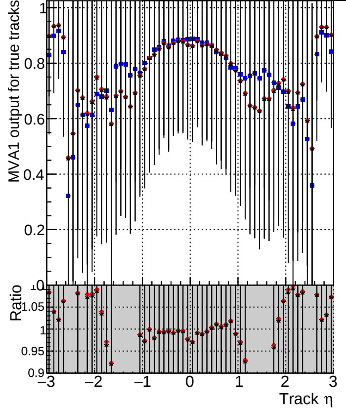
MVA1 of associated tracks (recoToSim) vs. track \eta Legend: DQM_V0001_R0000000001_Global_cmssw1000time_RECO (blue squares) DQM_V0001_R0000000001_Global_mkFitNewOLD1000time_RECO (red circles) DQM_V0001_R0000000001_Global_mkFitNewBins1DC1000time_RECO (black triangles)
