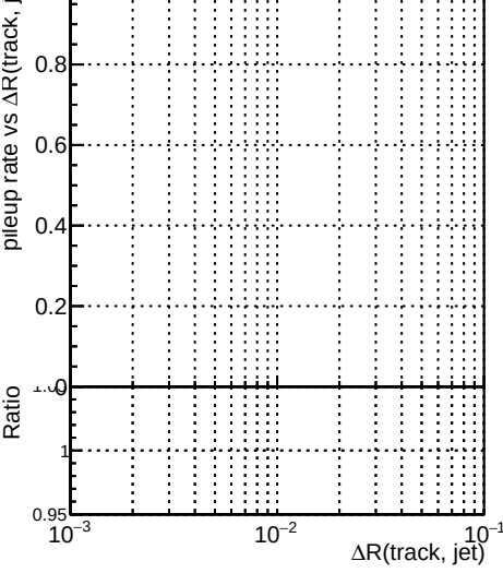
Pileup rate vs \Delta R(\text{track, jet})
