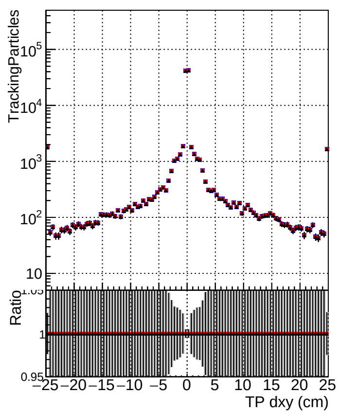
N of simulated track ■ DQM_V0001_R000000001 Global cmssw1000time RECO ● DQM_V0001_R000000001 Global mkFitNewOLD1000time RECO ▲ DQM_V0001_R000000001 Global mkFitNewTEST1000time RECO
