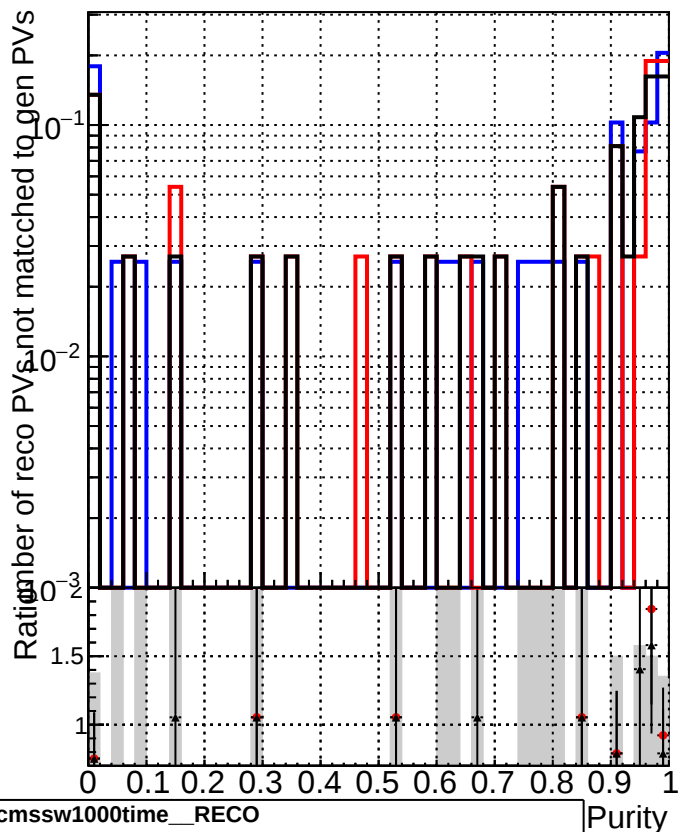
RecoPVAssoc2GenPVNotMatched_Purity
