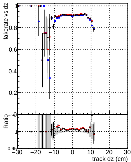
DOM V0001 R0000000001 Global cmssw1000time RECO DOM V0001 R0000000001 Global mktNewOldD1000time RECO DOM V0001 R0000000001 Global mktNewEST1000time RECO
