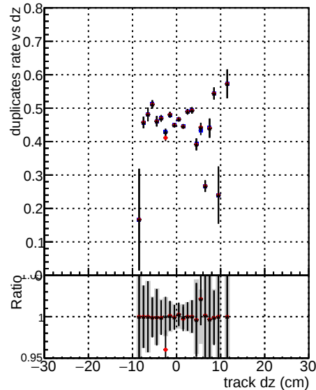
a mkFitNewOLD1000time RECO a mkFitNewTEST1000time RECO
