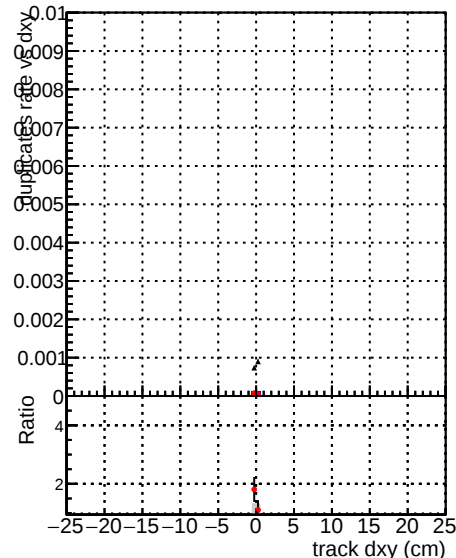
DOM V0001 R0000000001 Global cms-sw1000time RECO DOM V0001 R0000000001 Global mktFInewEST1000time RECO
