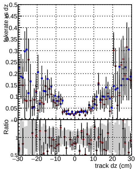
DOM V0001 R0000000001 Global cms-sw1000time RECO DOM V0001 R0000000001 Global mkFI-NewOLD1000time RECO DOM V0001 R0000000001 Global mkFI-NewTEST1000time RECO
