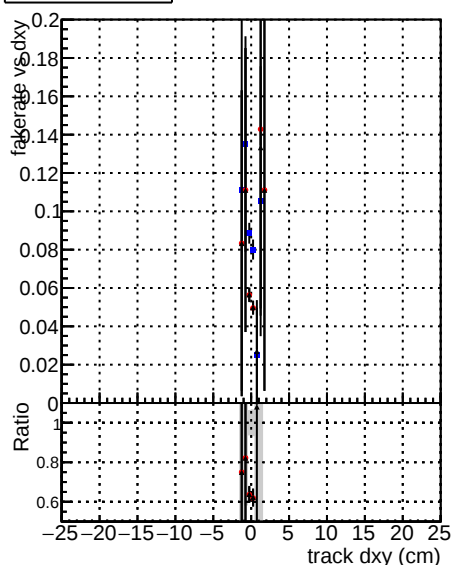
Legend for Fake rate vs dxy, Duplicates Rate vs Dxy, and Pileup rate vs dxy: DOM V0001 R0000000001 Global cms-sw1000time RECO DOM V0001 R0000000001 Global mktNewOLD1000time RECO DOM V0001 R0000000001 Global mktNewTEST1000time RECO
