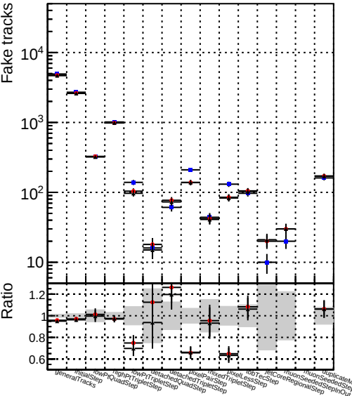
Number Legend Series Name Model Model Name DQM_V0001_R0000000001_Global_cmssw1000time_REC0 Global cmssw1000time_REC0 DQM_V0001_R0000000001_Global_mkFitNewOLD1000time_REC0 Global mkFitNewOLD1000time_REC0 DQM_V0001_R0000000001_Global_mkFitNewTEST1000time_REC0 Global mkFitNewTEST1000time_REC0
