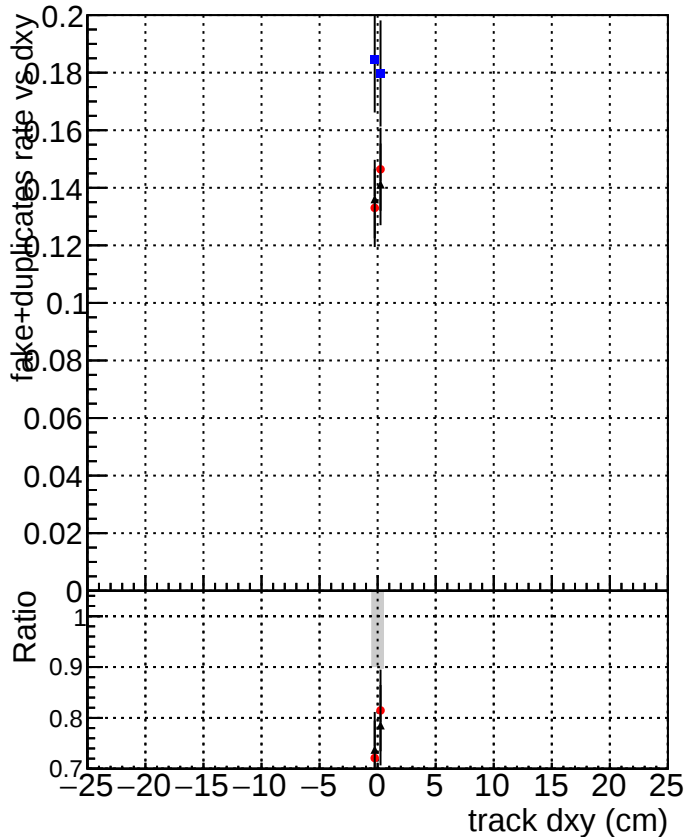
fake+duplicates rate vs dxy
