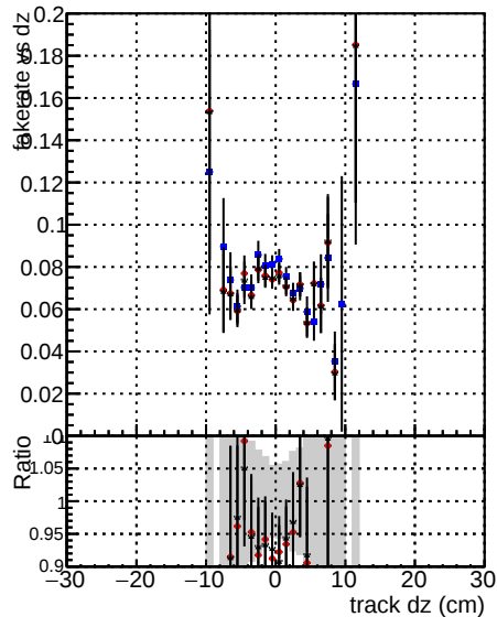
Fake rate vs d Legend DOM V0001 R0000000001 Global cmssw1000time RECO Blue dot DOM V0001 R0000000001 Global cmssw1000time RECO Red dot DOM V0001 R0000000001 Global mkFitNewOLD1000time RECO Black dot DOM V0001 R0000000001 Global mkFitNewTEST1000time RECO
