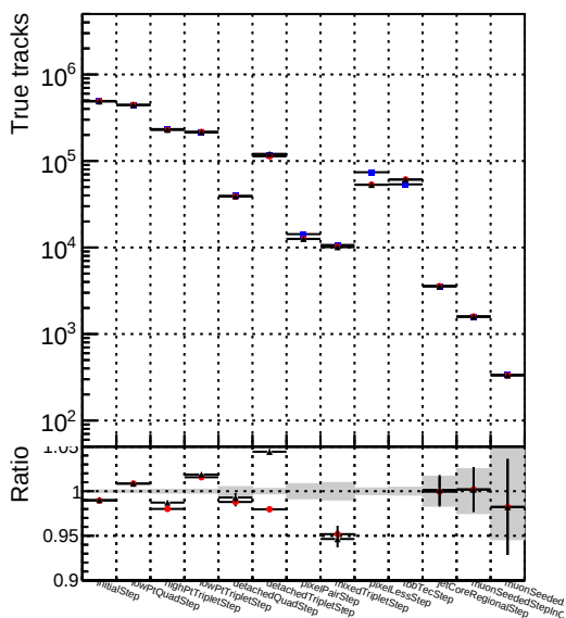
—●— DQM_V0001_R000000001_Global_cmssw1000time_RECO —●— DQM_V0001_R000000001_Global_mkFitNewOLD1000time_RECO —●— DQM_V0001_R000000001_Global_mkFitNewTEST1000time_RECO
