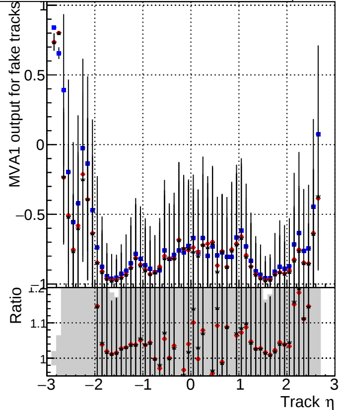
MVA1 of associated tracks (recoToSim) vs. track \eta ■ DQM_V0001_R000000001_Global_cmssw1000time_RECO ● DQM_V0001_R000000001_Global_mkFitNewOLD1000time_RECO ★ DQM_V0001_R000000001_Global_mkFitNewTEST1000time_RECO
