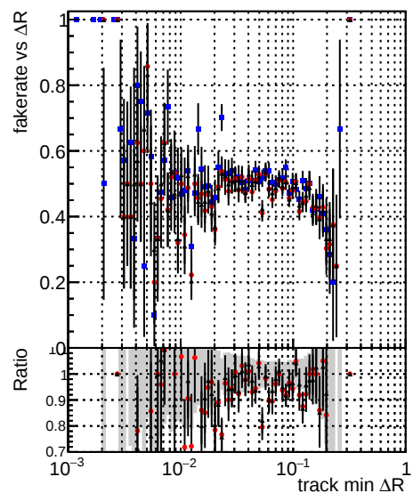
—●— DQM_V0001_R000000001_Global_cmssw1000time_RECO —●— DQM_V0001_R000000001_Global_mkFitNewOLD1000time_RECO —●— DQM_V0001_R000000001_Global_mkFitNewTEST1000time_RECO
