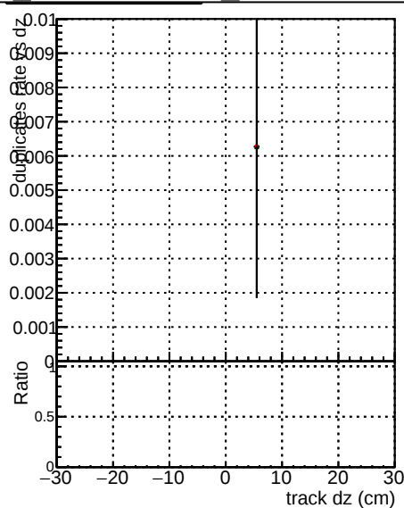
DOM V0001 R0000000001 Global cms-sw1000time RECO DOM V0001 R0000000001 Global mkFitNewOLD1000time RECO DOM V0001 R0000000001 Global mkFitNewSEED1000time RECO
