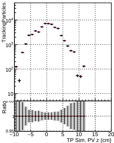
N of simulated tracks vs. sim PV z
