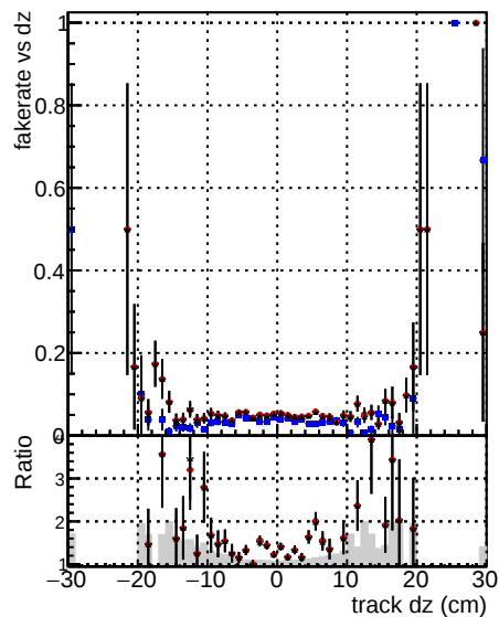
DOM V0001 R0000000001 Global cms-sw1000time RECO DOM V0001 R0000000001 Global mktInNewOLD1000time RECO DOM V0001 R0000000001 Global mktInNewSEED1000time RECO
