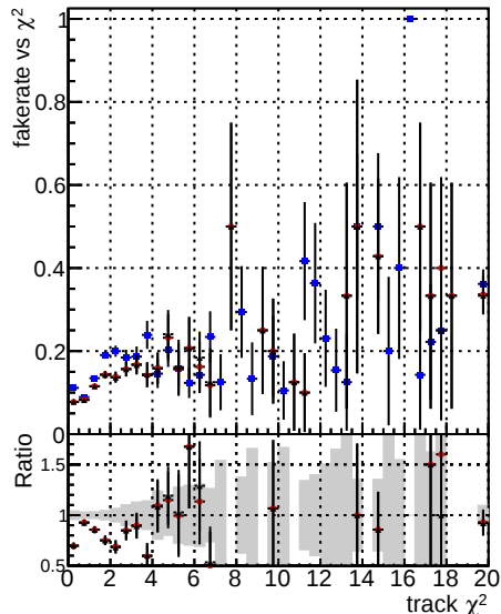
Fake rate vs. Legend Global cmssw1000time RECO Global mktInNewSEED1000time RECO Blue line with diamond DOM V0001 R0000000001 Red line with star DOM V0001 R0000000001
