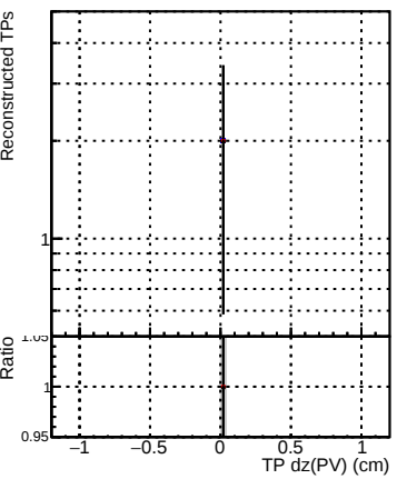
N of associated tracks (simToReco) vs dz(PV)
