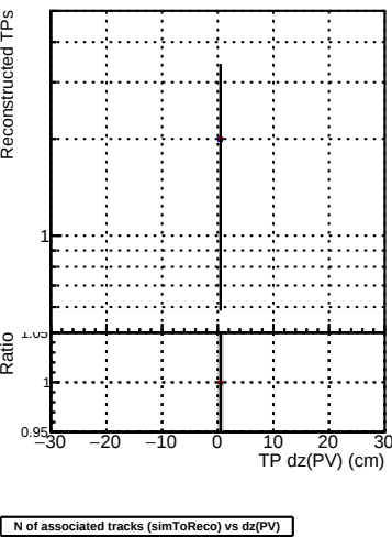
N of associated tracks (simToReco) vs dz(PV)
