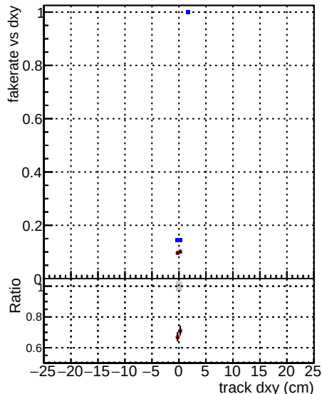
Legend for Fake rate vs d, Duplicates Rate vs Dxy, and Pileup rate vs dxy plots: DOM V0001 R0000000001 Global cms-sw1000time RECO DOM V0001 R0000000001 Global mktFitNewBP1000time RECO
