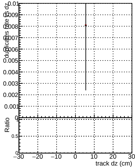
Global cmssw1000time RECO Global mkFitNewBOP1000time RECO
