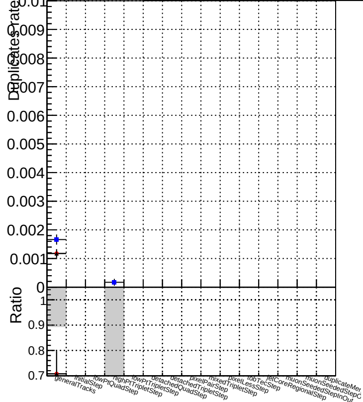
Duplicates rate vs collection Legend: ■ DQM_V0001_R000000001 Global cmssw1000time RECO ● DQM_V0001_R000000001 Global mkFitNewOLD1000time RECO ▲ DQM_V0001_R000000001 Global mkFitNewDUP1000time RECO
