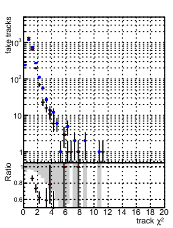
N of reco track vs. \chi^2 DGM V0001 R0000000000 Global mkFitNewDup1000time_REC0 Global mkFitNewDup1000time_REC0
