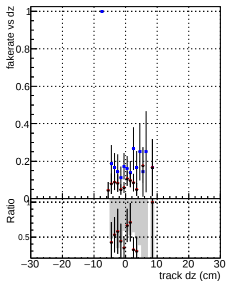
Fake rate vs d DOM_V0001_R0000000001 Global_cmssw1000time_REC0 DOM_V0001_R0000000001 Global_mktFitNewBOP1000time_REC0
