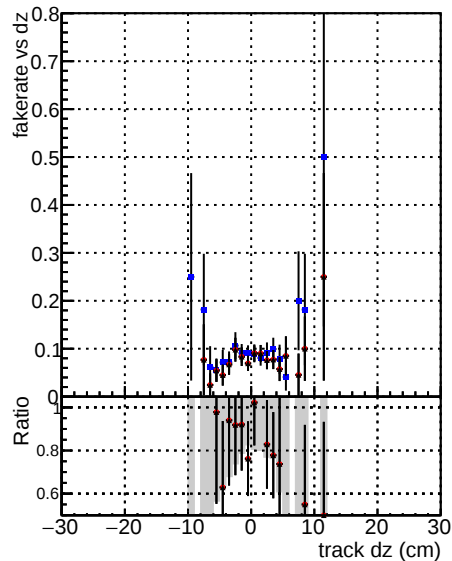
DOM V0001 RECO Global cms-sw1000time RECO DOM V0001 RECO Global mkFitNewBOP1000time RECO
