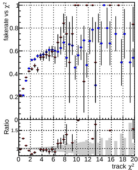
Fake rate vs. DOM V0001 R0000000001 Global cms-sw1000time RECO DOM V0001 R0000000001 Global mkFitNewBOP1000time RECO
