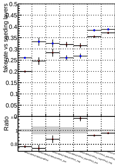
Fake rate vs. DOM V0001 R0000000001 Global cms-sw1000time RECO DOM V0001 R0000000001 Global mkFitNewBOP1000time RECO
