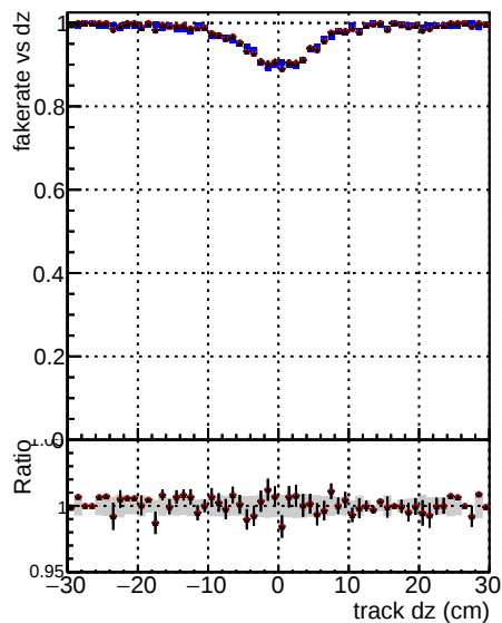
Legend: DOM V0001 R0000000001 Global cms-sw1000time RECO BCM V0001 R0000000001 Global mkFitNewBOP1000time RECO
