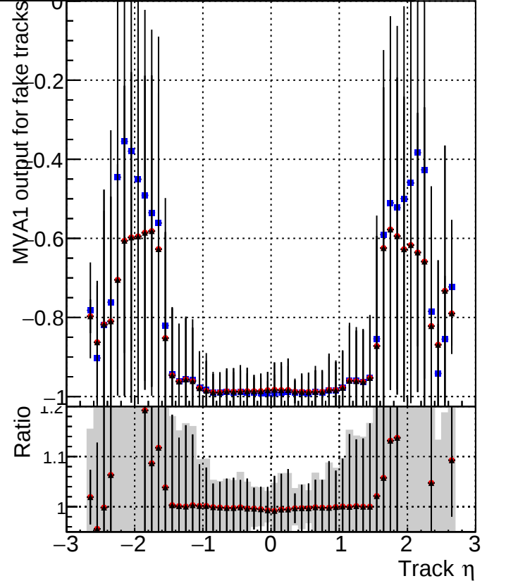
MVA1 of associated tracks (recoToSim) vs. track \eta ■ DQM_V0001_R0000000001_Global_cmssw1000time_RECO ● DQM_V0001_R0000000001_Global_mkFitNewOLD1000time_RECO ▲ DQM_V0001_R0000000001_Global_mkFitNewDUP1000time_RECO
