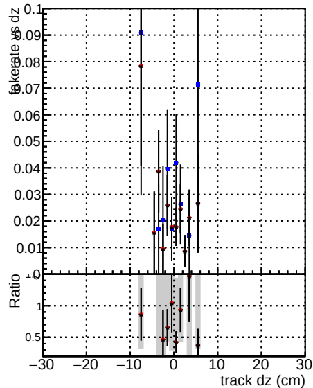
Fake rate vs dz DOM V0001 R0000000001 Global cms-sw1000time RECO DOM V0001 R0000000001 Global mktFitNewBOP1000time RECO
