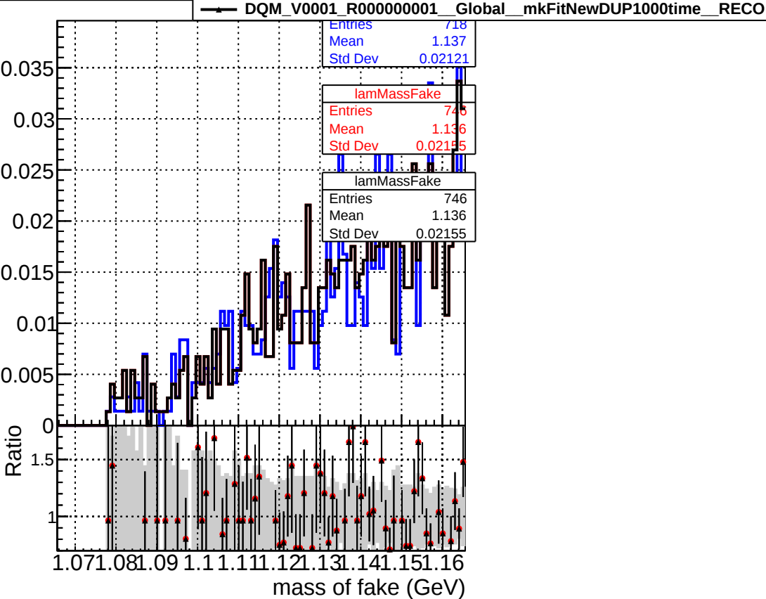
Mass of fake Lambda
