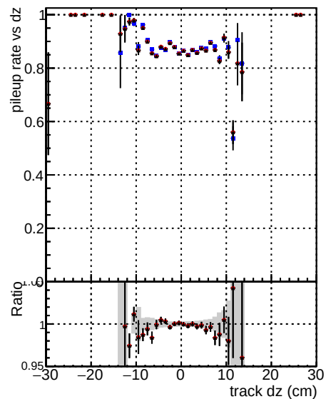
Global mkFitNewBOP1000time RECO
