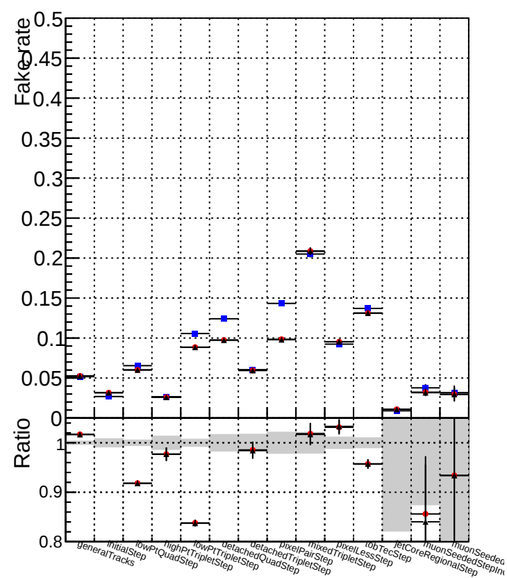
Fakerrate vs collection
