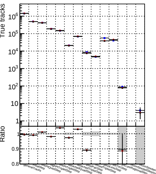
Number Legend Series Name Series Description DQM_V0001_R0000000001_Global_cmssw1000time_RECO DQM_V0001_R0000000001_Global_mkFitNewOLD1000time_RECO DQM_V0001_R0000000001_Global_mkFitNewALL1000time_RECO
