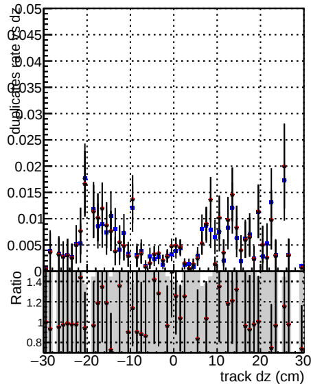
Global cmssw1000time RECO
