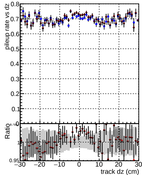
Global mkFitNewALL1000time RECO
